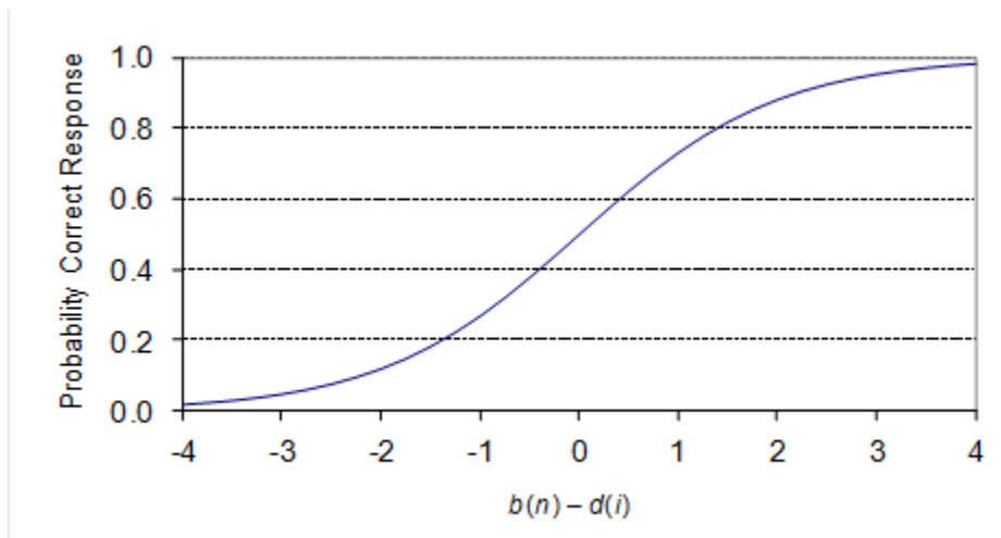
Figure 10. The Rasch Model--the probability person n responds correctly to item i .
