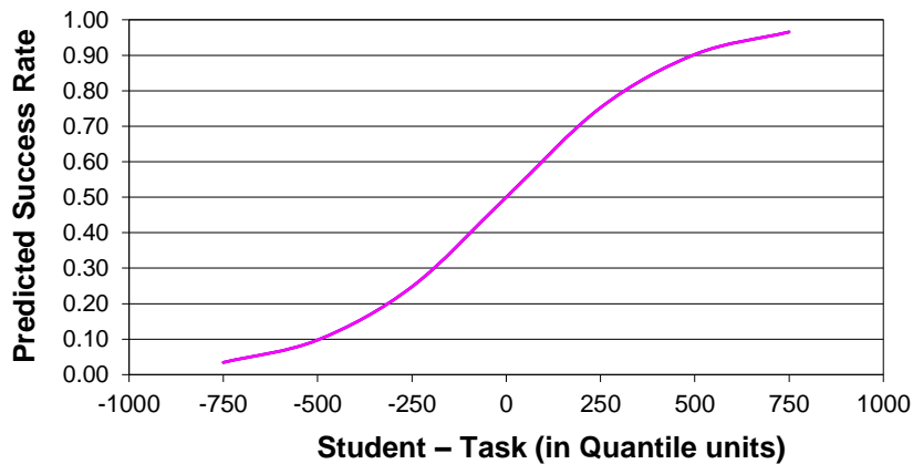
Figure 9. Student-mathematical demand discrepancy and predicted success rate.
