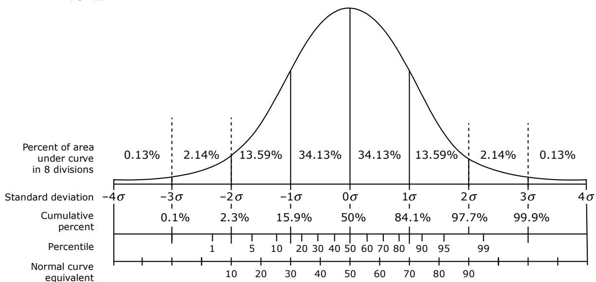
Figure 8. Normal distribution of scores described in scale scores, percentiles, stanines, and NCEs.
