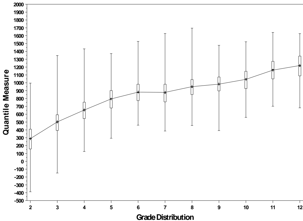
Figure 3. Box-and-whisker plots of the Rasch ability estimates for the final sample of students with outfit statistics less than 1.8 (N = 9,176).
