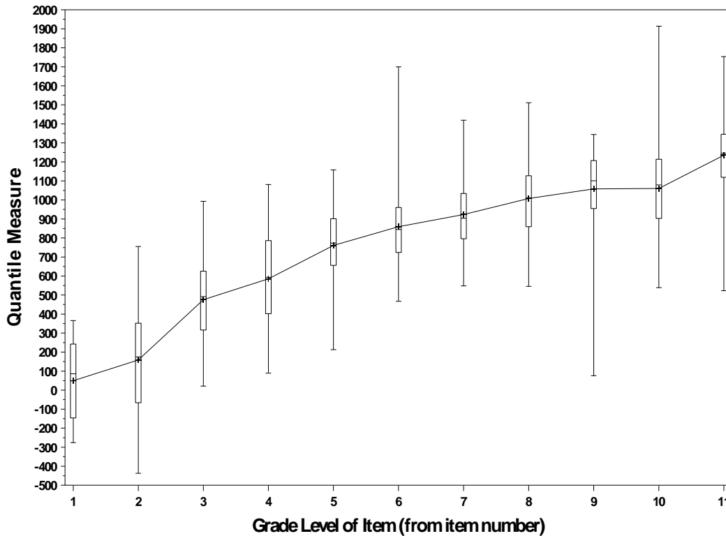
Figure 4. Box-and-whisker plots of the Rasch difficulty estimates of the 685 Quantile Framework items for the final sample of students ( N = 9,176 ).
