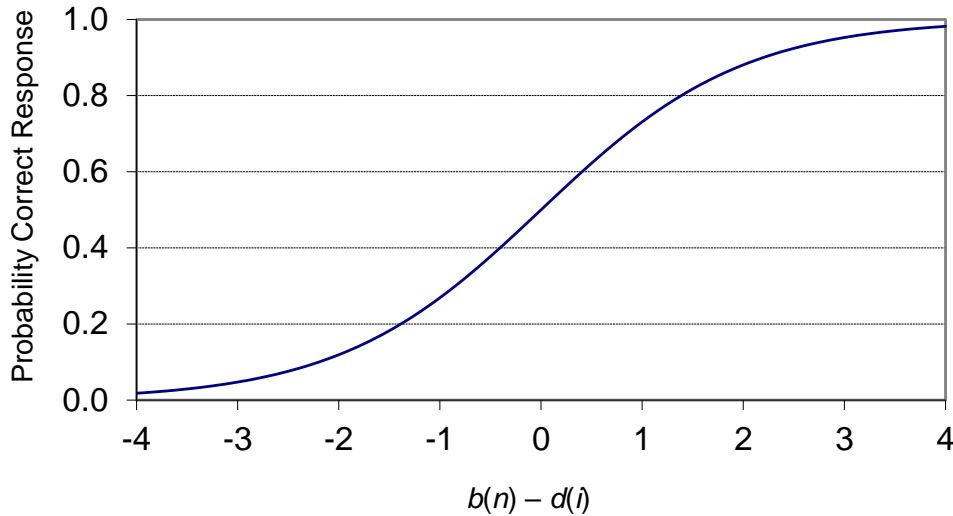
Figure 1. The Rasch Model—the probability person n responds correctly to item i .
